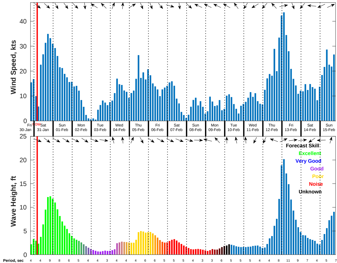
Wind & Wave Forecast for NDBC 42036 from 30-Jan-2026 19:00:00 to 15-Feb-2026 19:00:00
