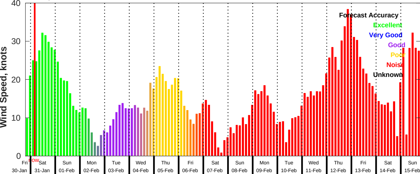
GFS Wind Speed Forecast for NDBC 42040 from 30-Jan-2026 19:00:00 to 15-Feb-2026 19:00:00
