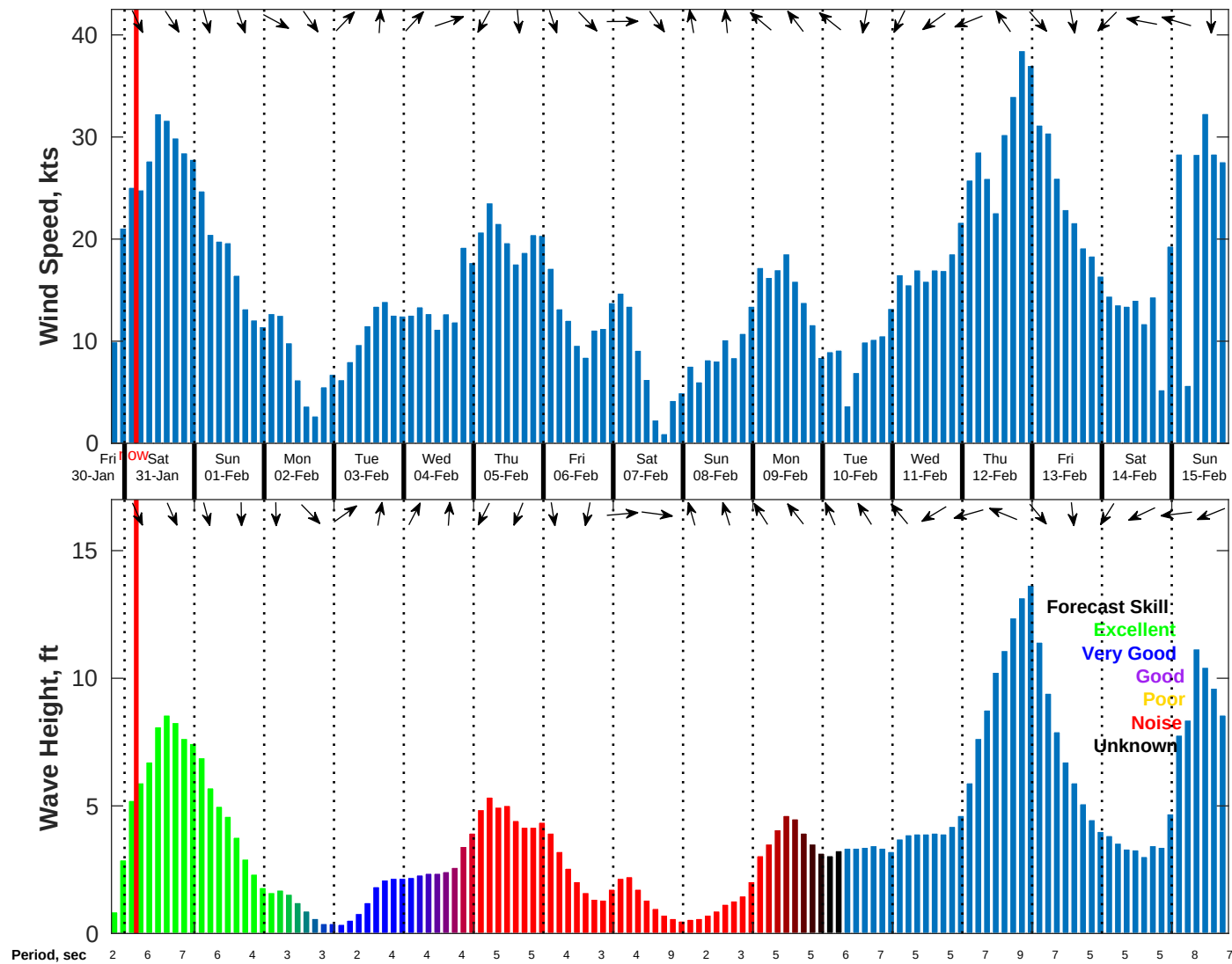
Wind & Wave Forecast for NDBC 42040 from 30-Jan-2026 19:00:00 to 15-Feb-2026 19:00:00
