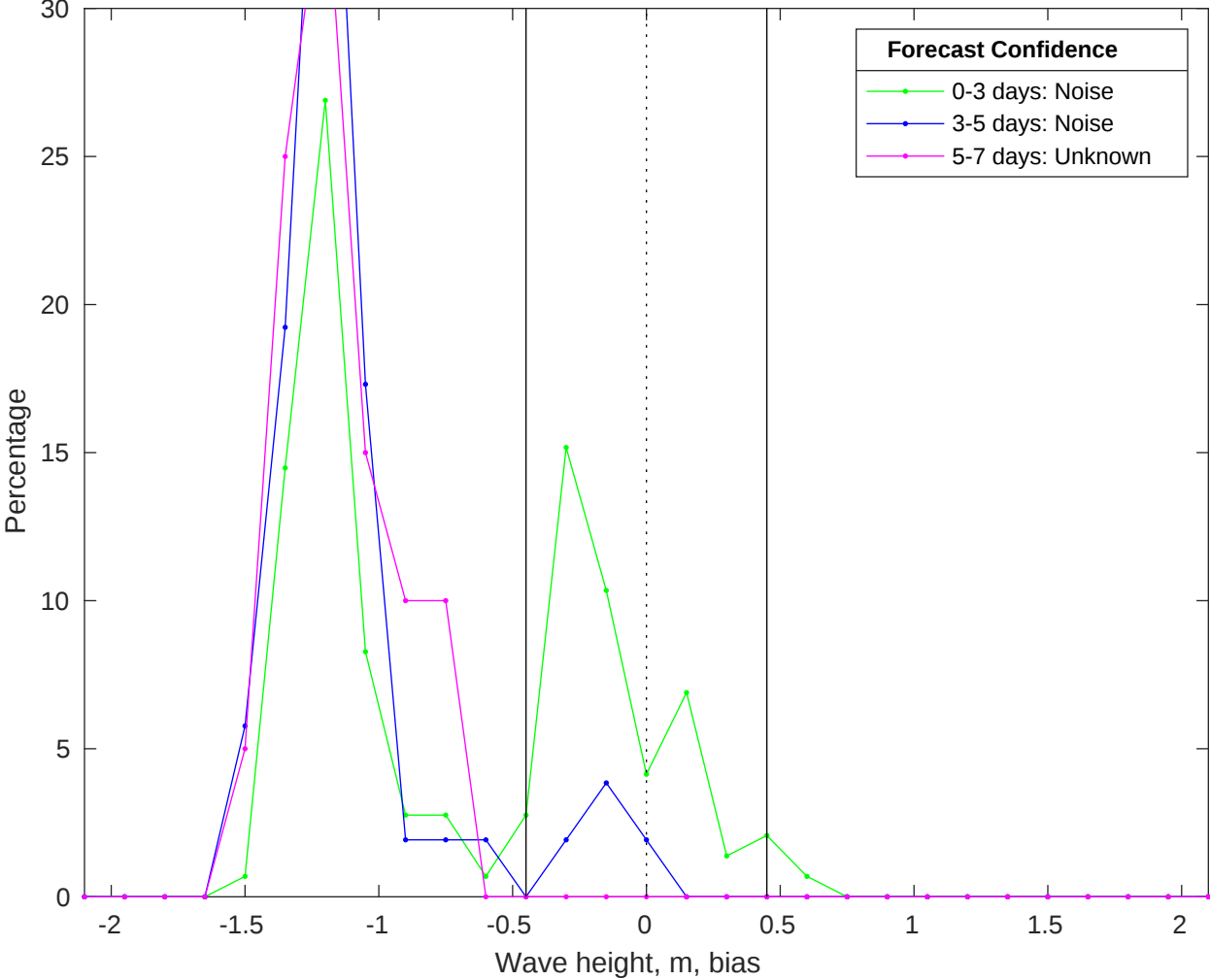
NDBC 42058 vs CMEMS Waves Bias Histogram: 30-Jan-2026
