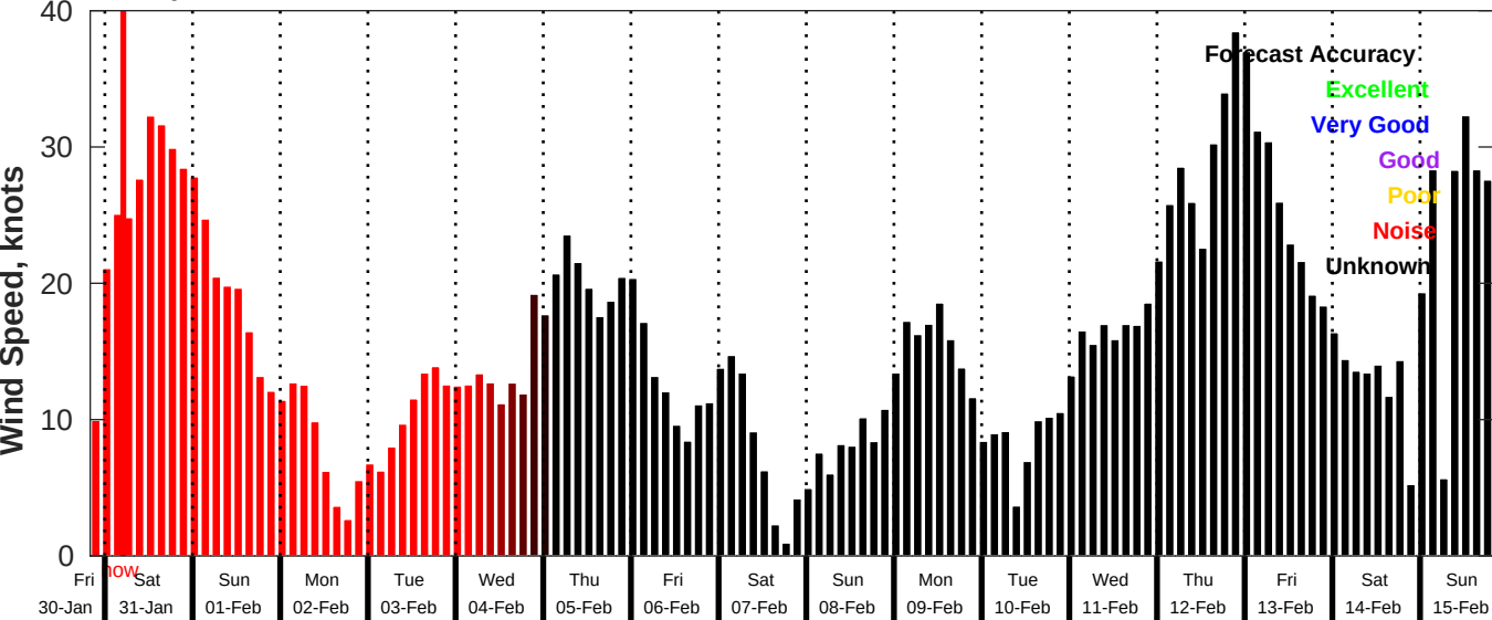
GFS Wind Speed Forecast for NDBC 42058 from 30-Jan-2026 20:00:00 to 15-Feb-2026 20:00:00
