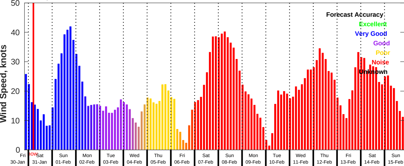
GFS Wind Speed Forecast for NDBC 44008 from 30-Jan-2026 20:00:00 to 15-Feb-2026 20:00:00
