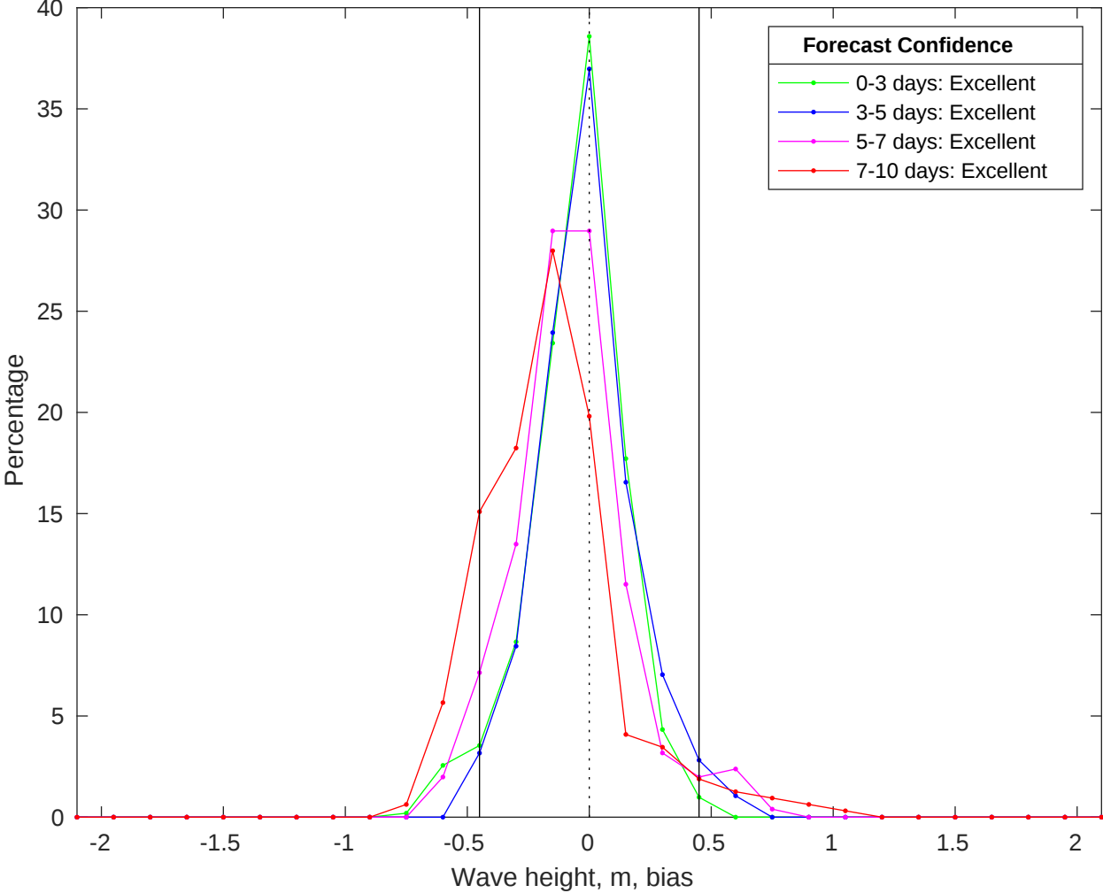
NDBC 46011 vs CMEMS Waves Bias Histogram: 31-Jan-2026
