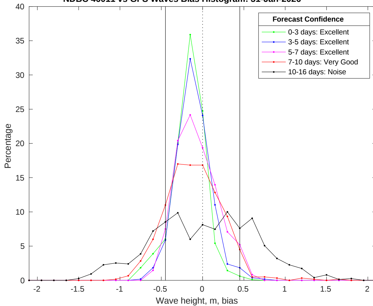
NDBC 46011 vs GFS Waves Bias Histogram: 31-Jan-2026
