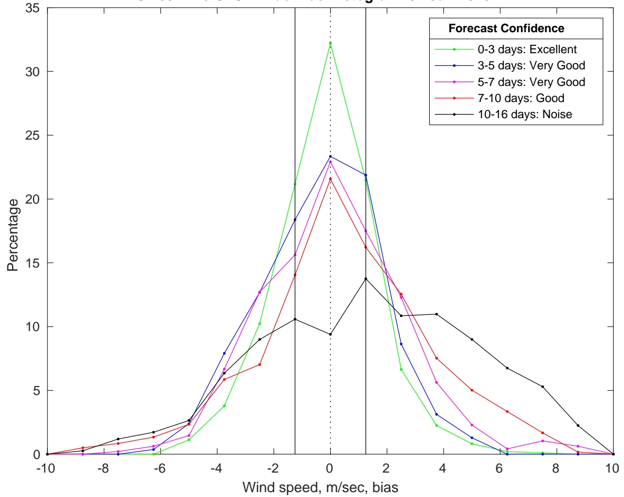
NDBC 46011 vs GFS Winds Bias Histogram: 31-Jan-2026
