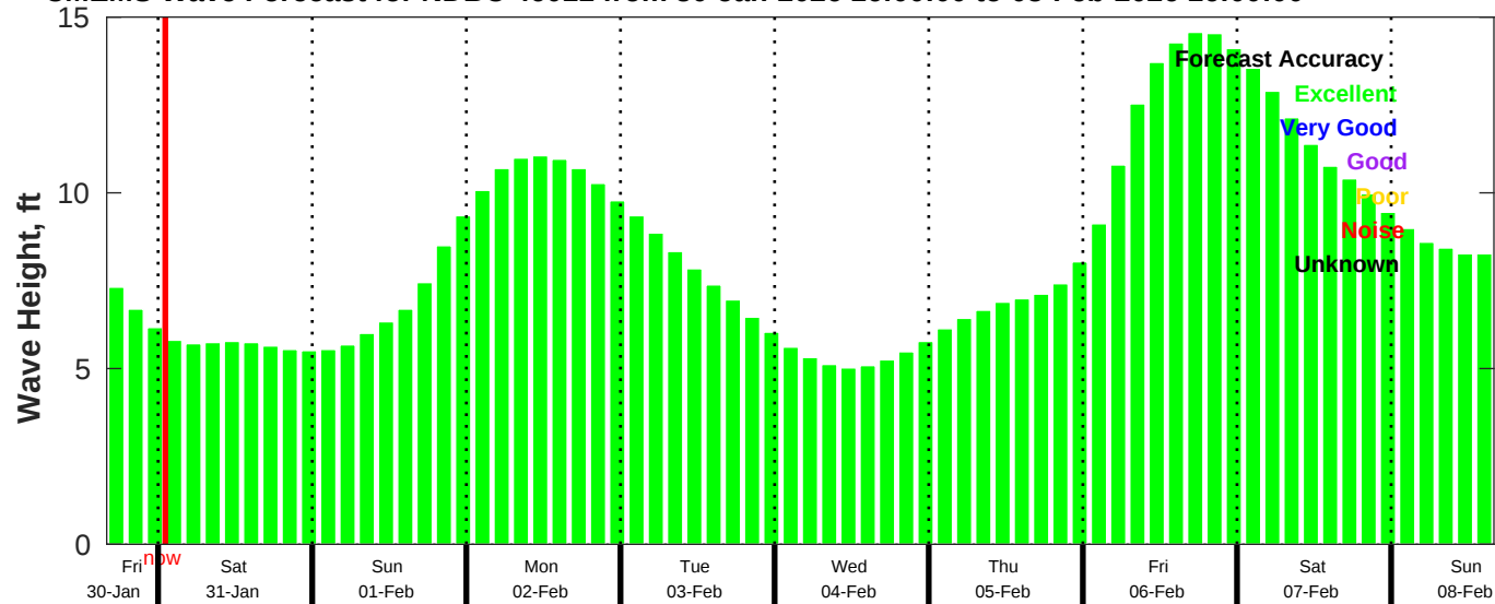
CMEMS Wave Forecast for NDBC 46011 from 30-Jan-2026 16:00:00 to 08-Feb-2026 16:00:00
