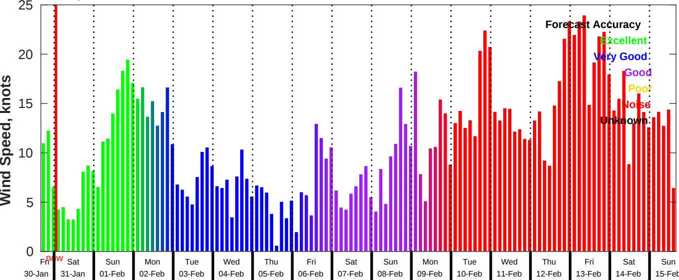
GFS Wind Speed Forecast for NDBC 46011 from 30-Jan-2026 16:00:00 to 15-Feb-2026 16:00:00
