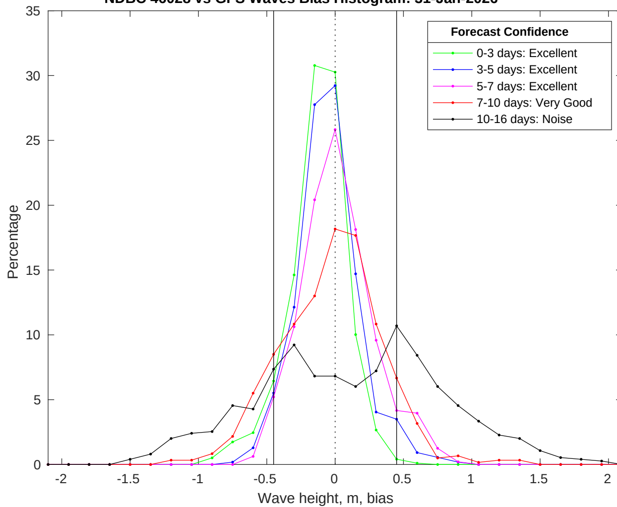
NDBC 46028 vs GFS Waves Bias Histogram: 31-Jan-2026
