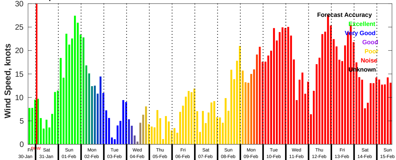
GFS Wind Speed Forecast for NDBC 46028 from 30-Jan-2026 16:00:00 to 15-Feb-2026 16:00:00
