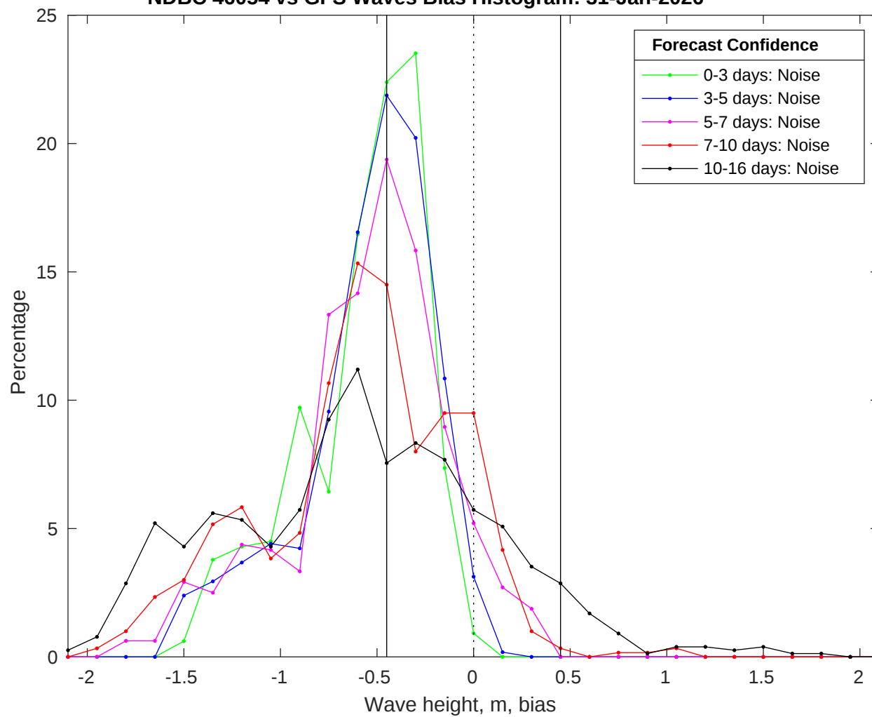
NDBC 46054 vs GFS Waves Bias Histogram: 31-Jan-2026
