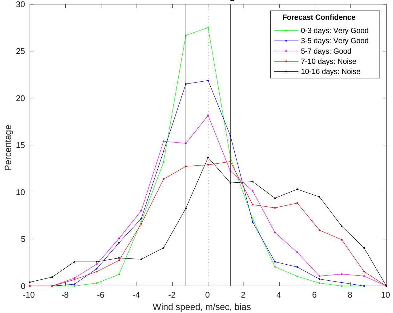
NDBC 46054 vs GFS Winds Bias Histogram: 31-Jan-2026
