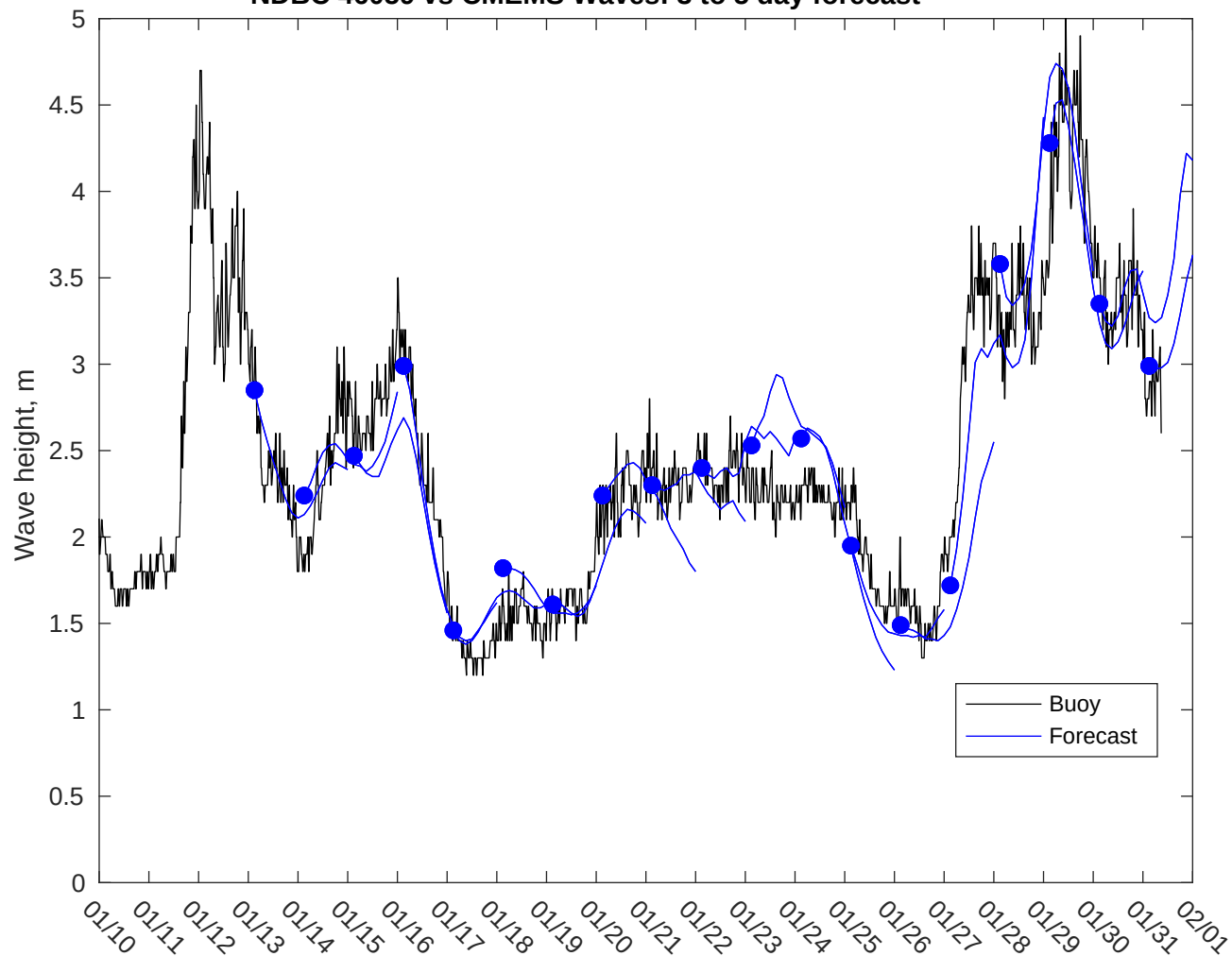
NDBC 46059 vs CMEMS Waves: 3 to 5 day forecast
