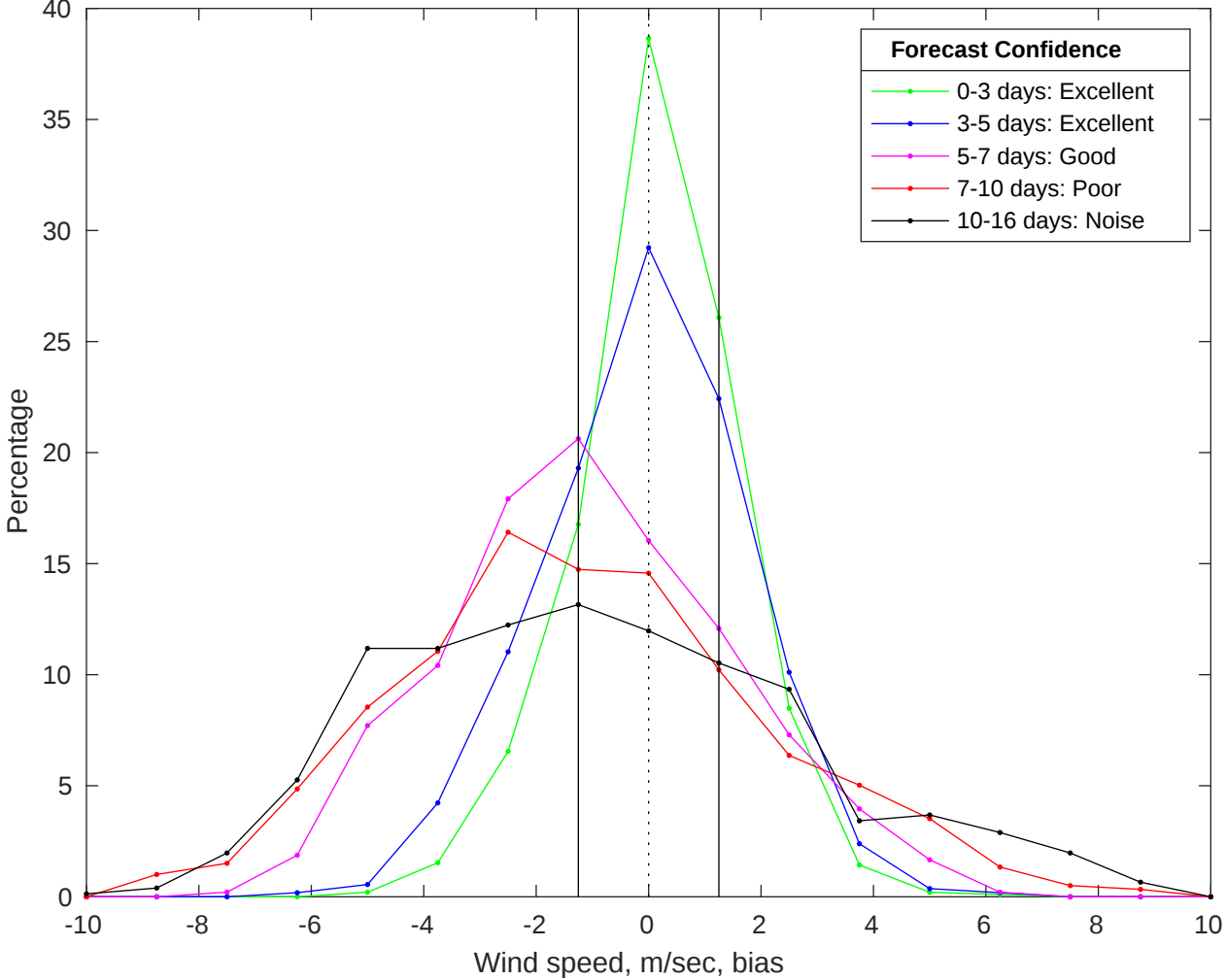
NDBC 46059 vs GFS Winds Bias Histogram: 31-Jan-2026
