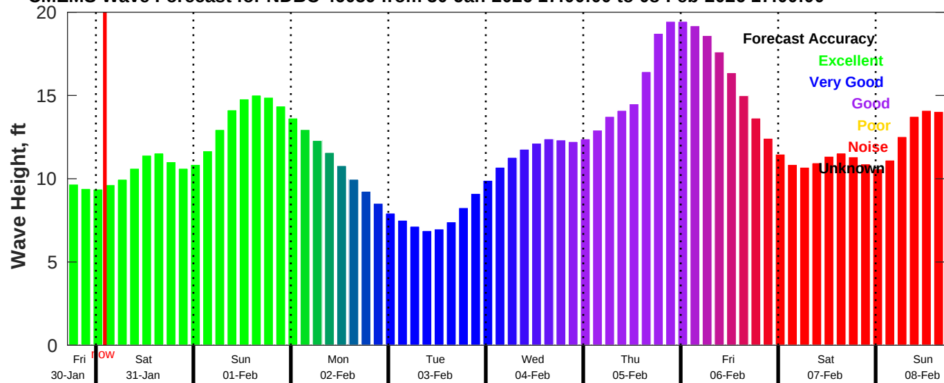
CMEMS Wave Forecast for NDBC 46059 from 30-Jan-2026 17:00:00 to 08-Feb-2026 17:00:00
