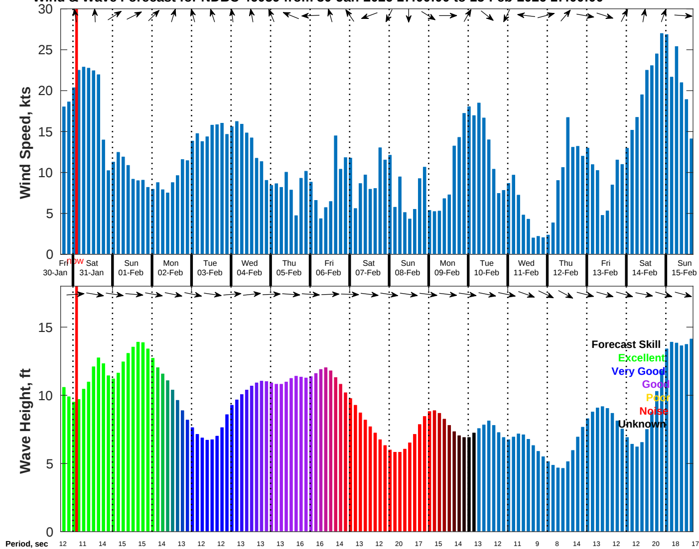
Wind & Wave Forecast for NDBC 46059 from 30-Jan-2026 17:00:00 to 15-Feb-2026 17:00:00
