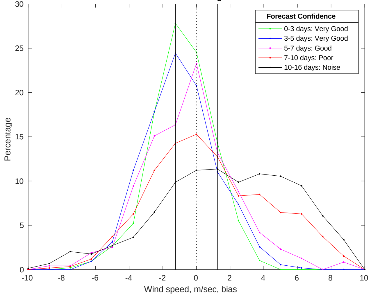
NDBC 46069 vs GFS Winds Bias Histogram: 31-Jan-2026
