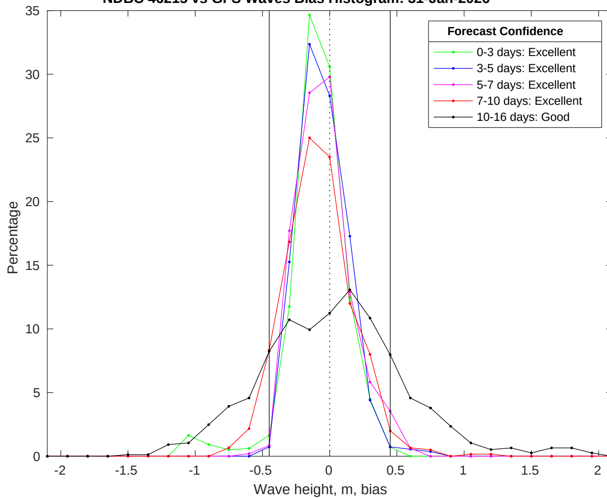
NDBC 46215 vs GFS Waves Bias Histogram: 31-Jan-2026
