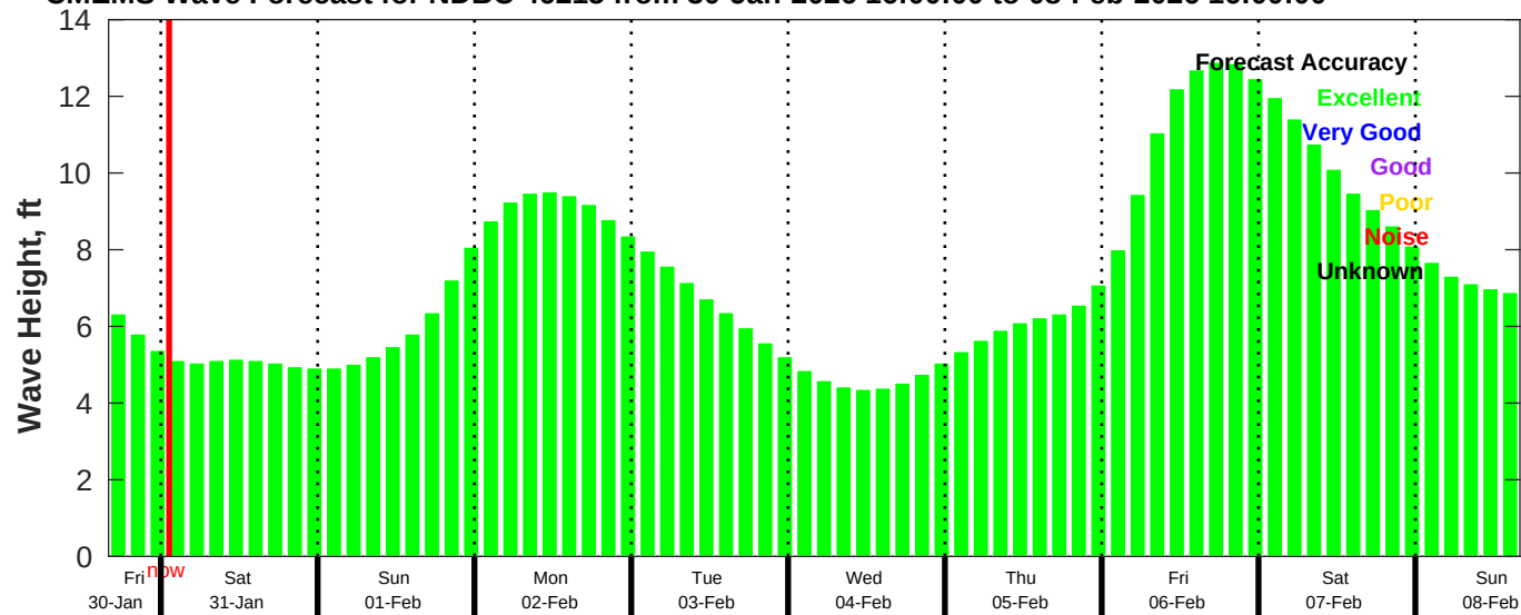
CMEMS Wave Forecast for NDBC 46215 from 30-Jan-2026 16:00:00 to 08-Feb-2026 16:00:00
