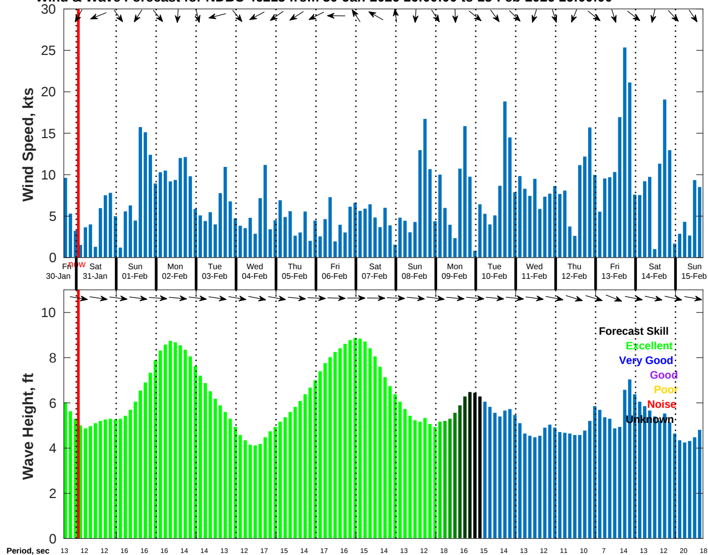
Wind & Wave Forecast for NDBC 46215 from 30-Jan-2026 16:00:00 to 15-Feb-2026 16:00:00
