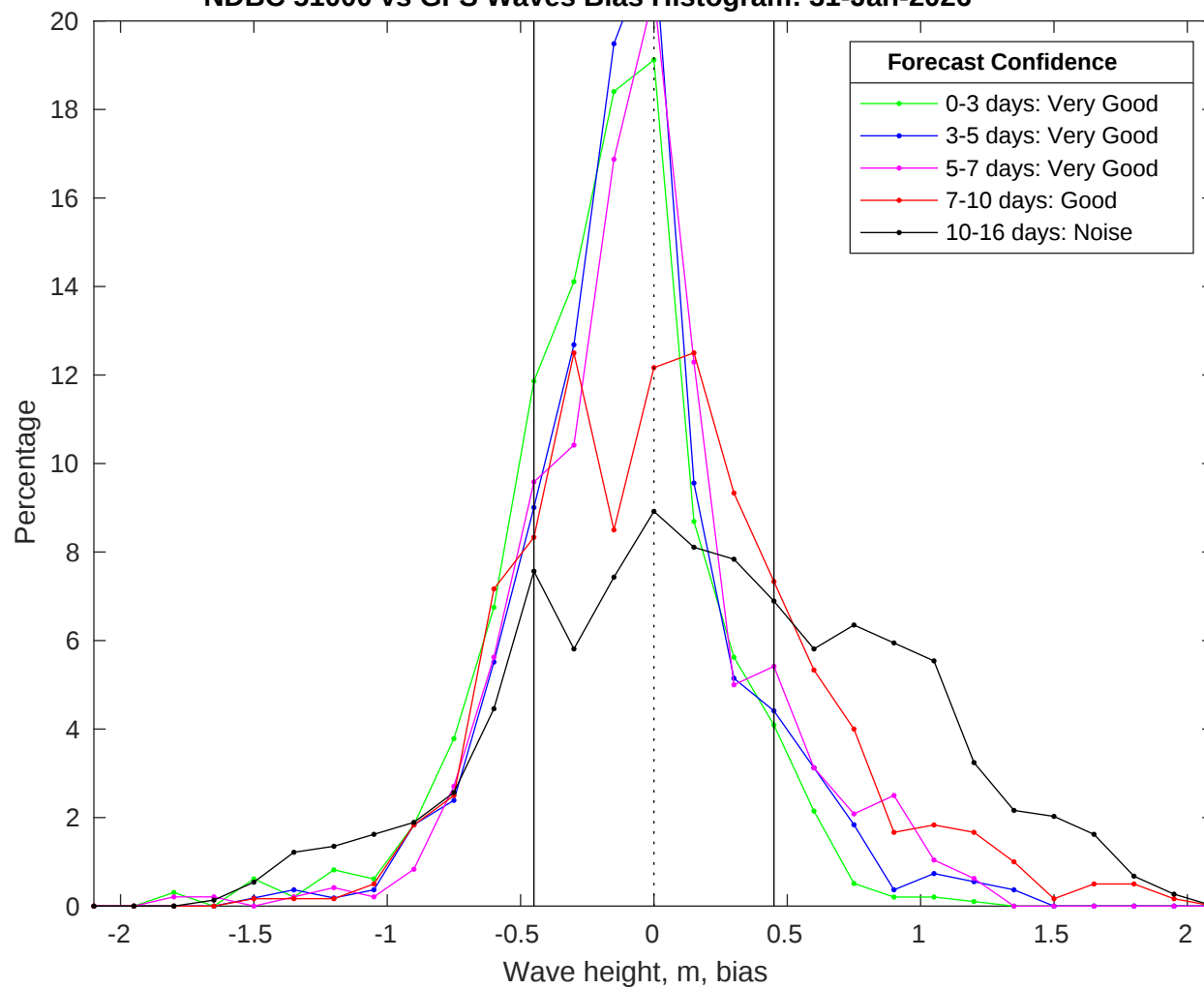
NDBC 51000 vs GFS Waves Bias Histogram: 31-Jan-2026
