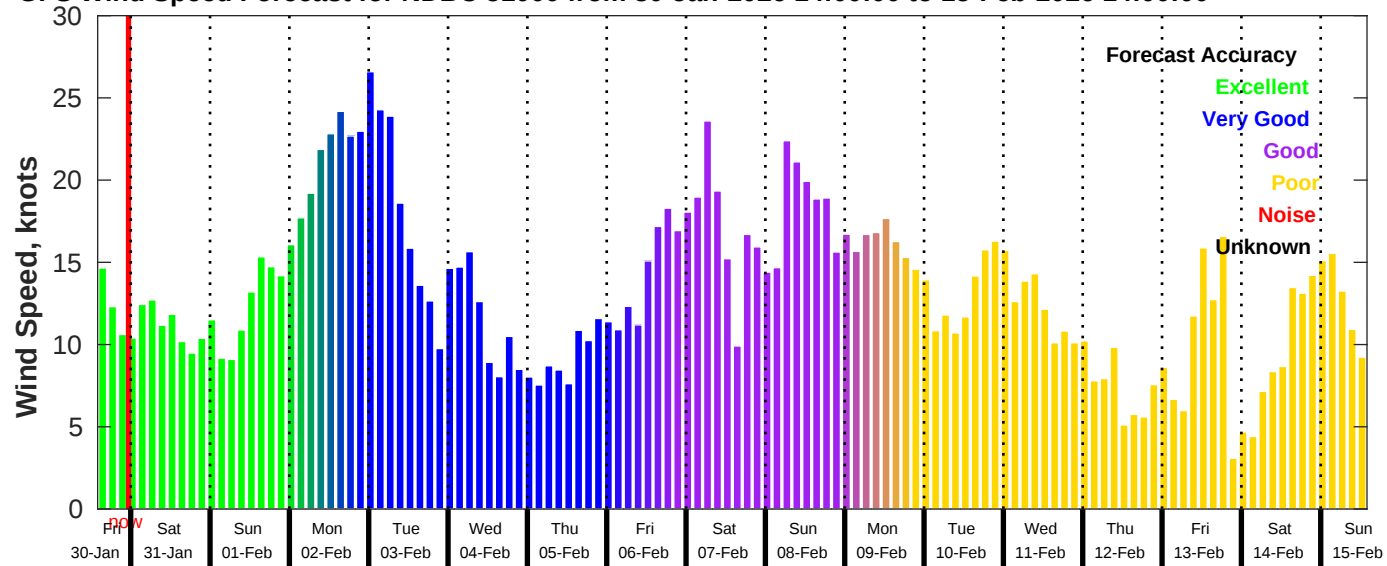
GFS Wind Speed Forecast for NDBC 51000 from 30-Jan-2026 14:00:00 to 15-Feb-2026 14:00:00
