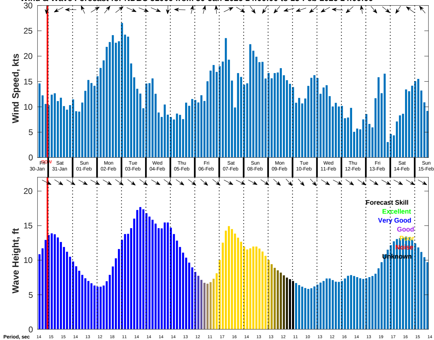
Wind & Wave Forecast for NDBC 51000 from 30-Jan-2026 14:00:00 to 15-Feb-2026 14:00:00
