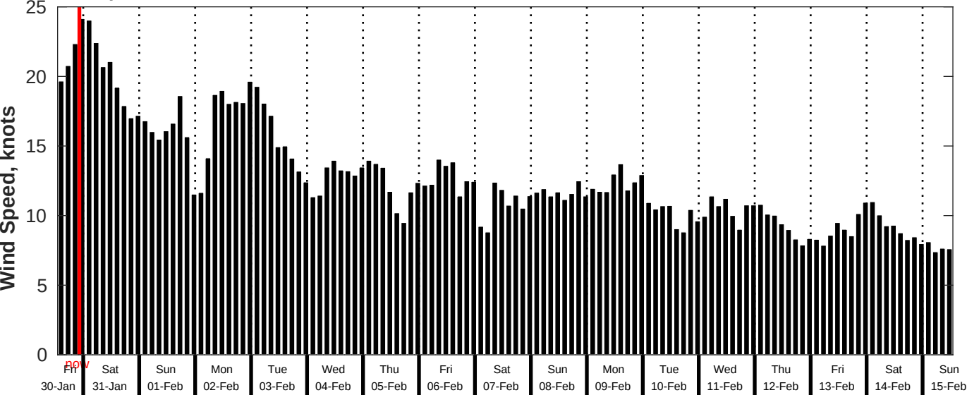
GFS Wind Speed Forecast for NDBC 51209 from 30-Jan-2026 13:00:00 to 15-Feb-2026 13:00:00
