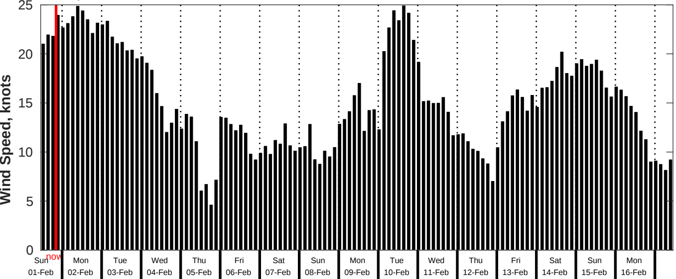
GFS Wind Speed Forecast for NDBC 52211 from 31-Jan-2026 11:00:00 to 16-Feb-2026 11:00:00
