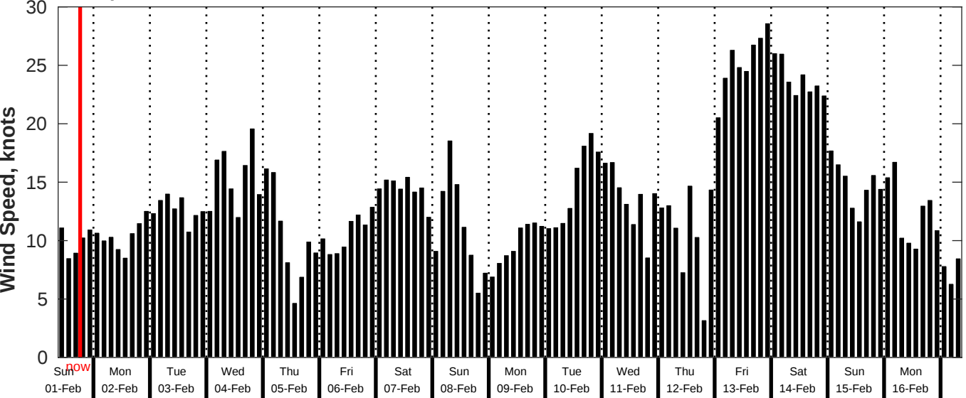
GFS Wind Speed Forecast for NDBC 52212 from 31-Jan-2026 09:00:00 to 16-Feb-2026 09:00:00
