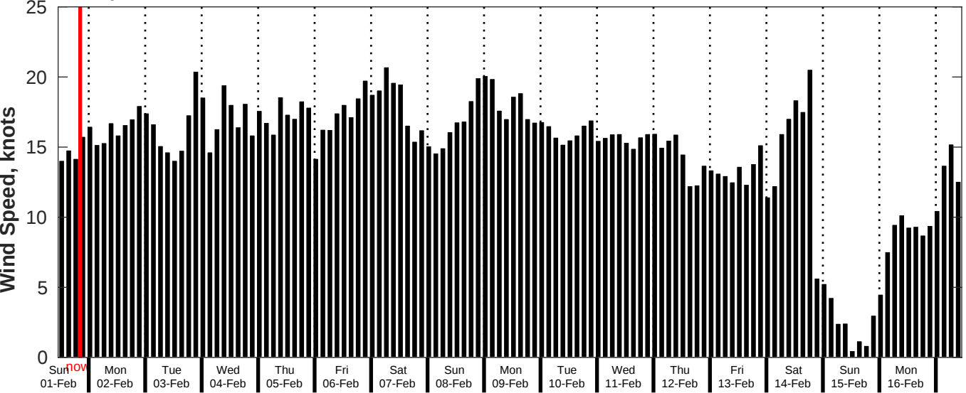
GFS Wind Speed Forecast for NDBC 52213 from 31-Jan-2026 11:00:00 to 16-Feb-2026 11:00:00
