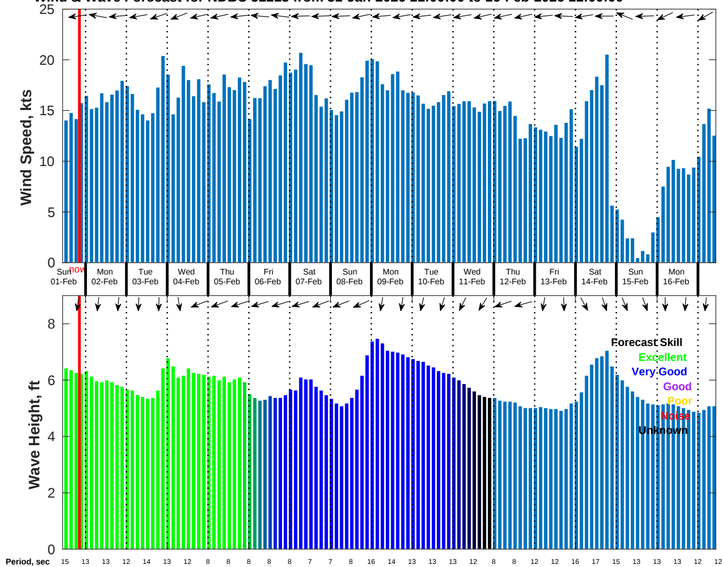
Wind & Wave Forecast for NDBC 52213 from 31-Jan-2026 11:00:00 to 16-Feb-2026 11:00:00
