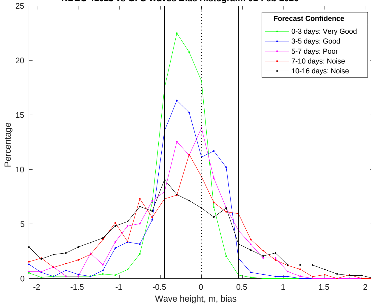
NDBC 41013 vs GFS Waves Bias Histogram: 01-Feb-2026
