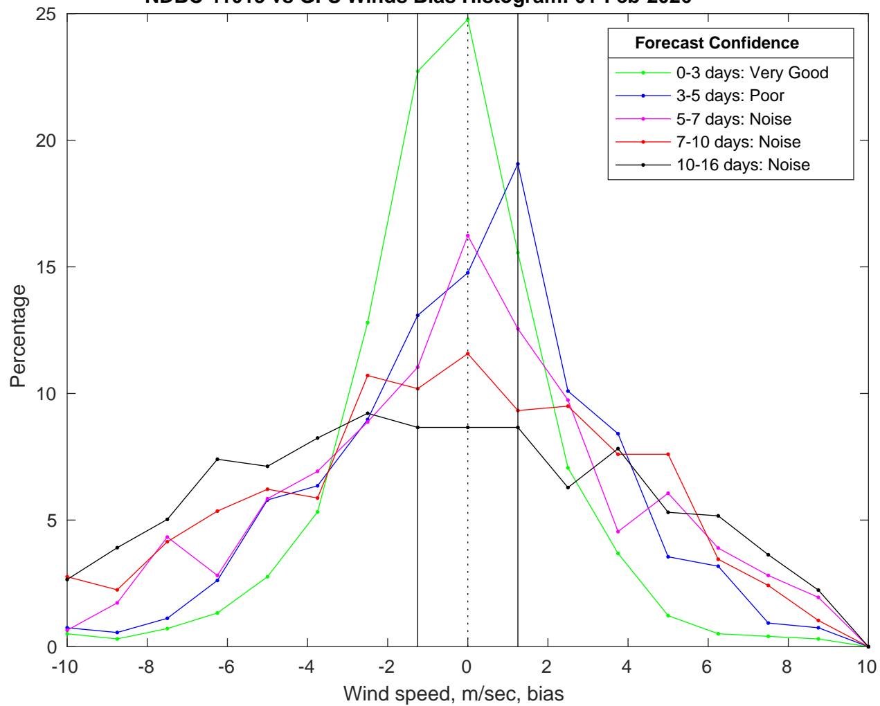
NDBC 41013 vs GFS Winds Bias Histogram: 01-Feb-2026
