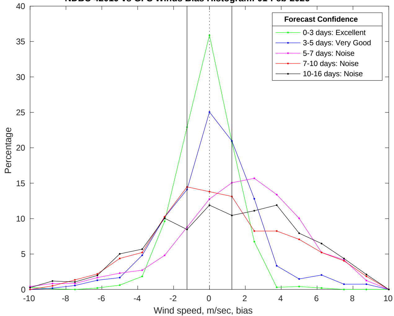
NDBC 42019 vs GFS Winds Bias Histogram: 01-Feb-2026
