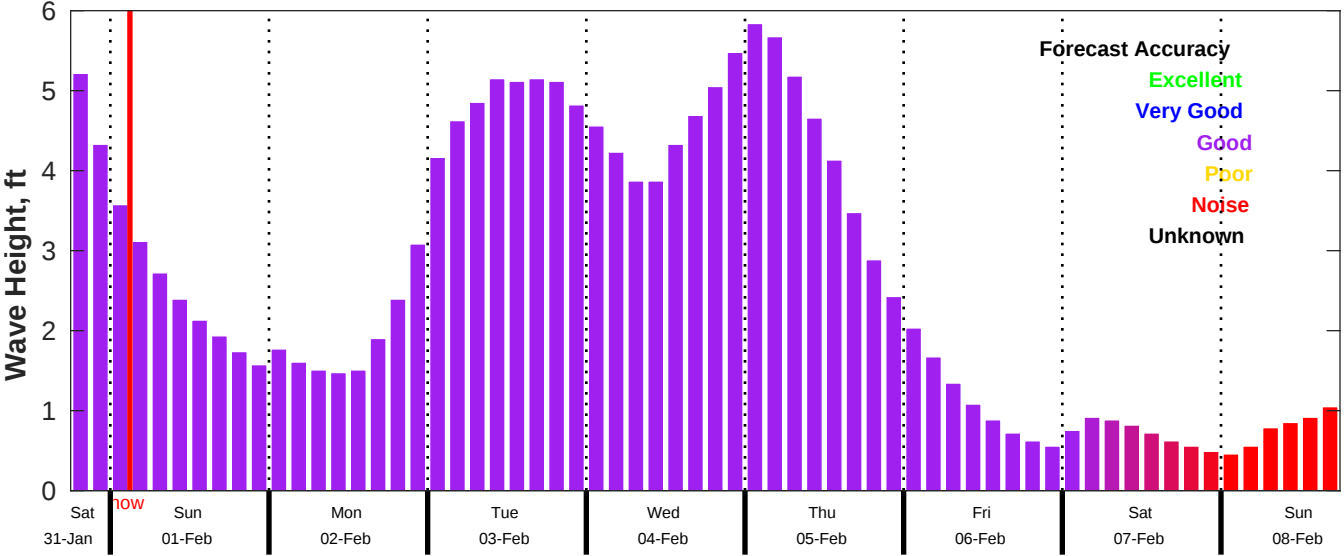
CMEMS Wave Forecast for NDBC 42019 from 31-Jan-2026 18:00:00 to 08-Feb-2026 18:00:00
