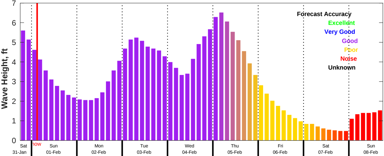
CMEMS Wave Forecast for NDBC 42020 from 31-Jan-2026 18:00:00 to 08-Feb-2026 18:00:00
