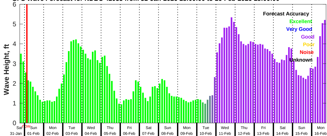
GFS Wave Forecast for NDBC 42035 from 31-Jan-2026 18:00:00 to 16-Feb-2026 18:00:00
