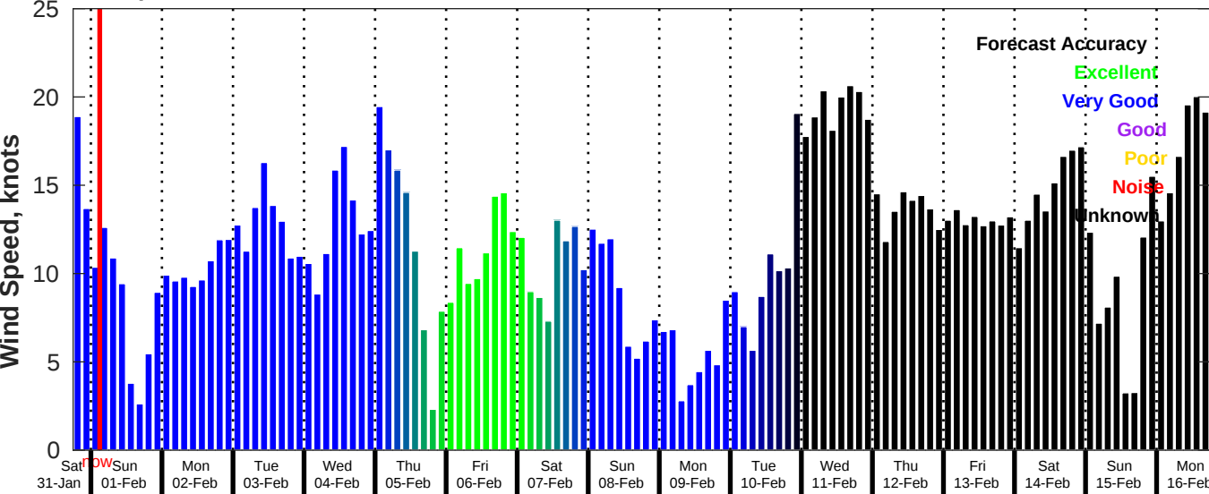
GFS Wind Speed Forecast for NDBC 42035 from 31-Jan-2026 18:00:00 to 16-Feb-2026 18:00:00
