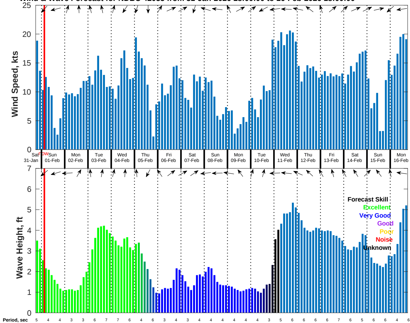
Wind & Wave Forecast for NDBC 42035 from 31-Jan-2026 18:00:00 to 16-Feb-2026 18:00:00
