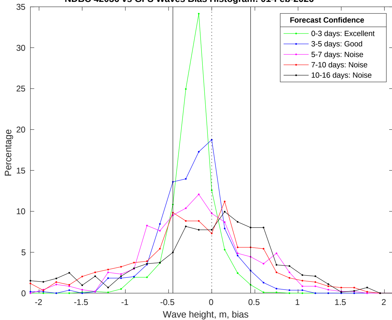
NDBC 42036 vs GFS Waves Bias Histogram: 01-Feb-2026
