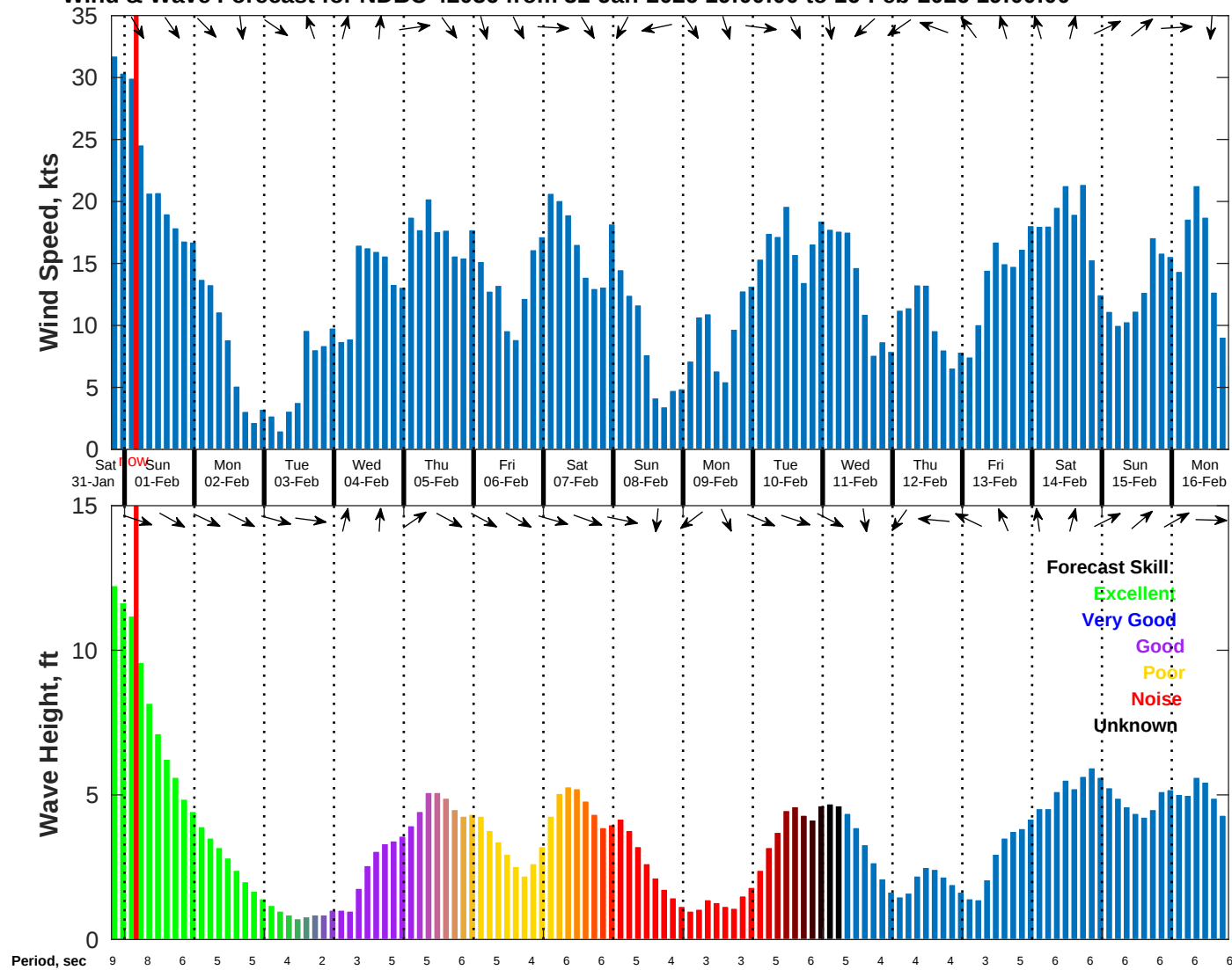
Wind & Wave Forecast for NDBC 42036 from 31-Jan-2026 19:00:00 to 16-Feb-2026 19:00:00
