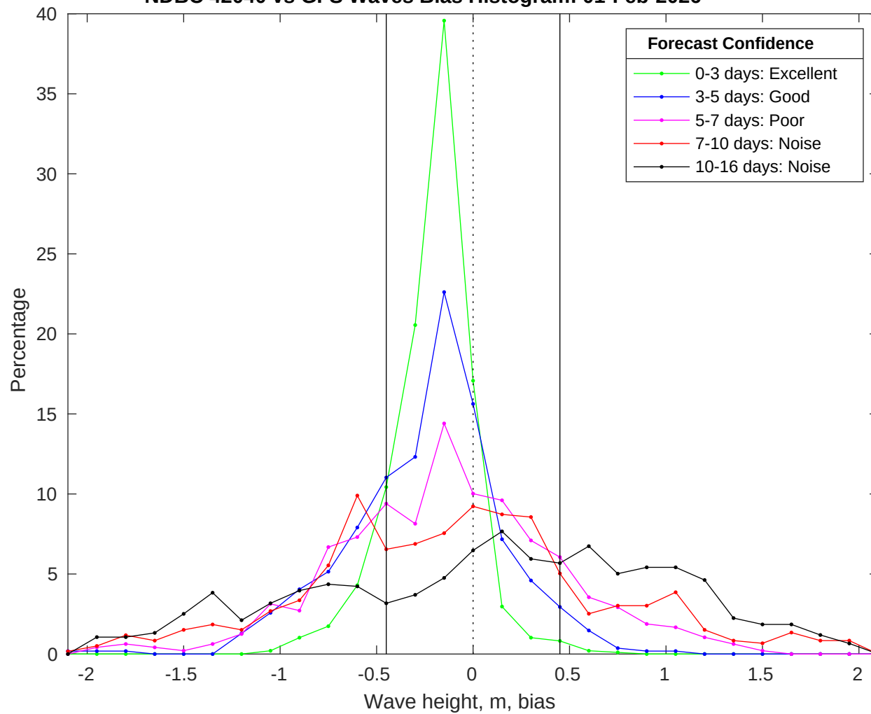
NDBC 42040 vs GFS Waves Bias Histogram: 01-Feb-2026
