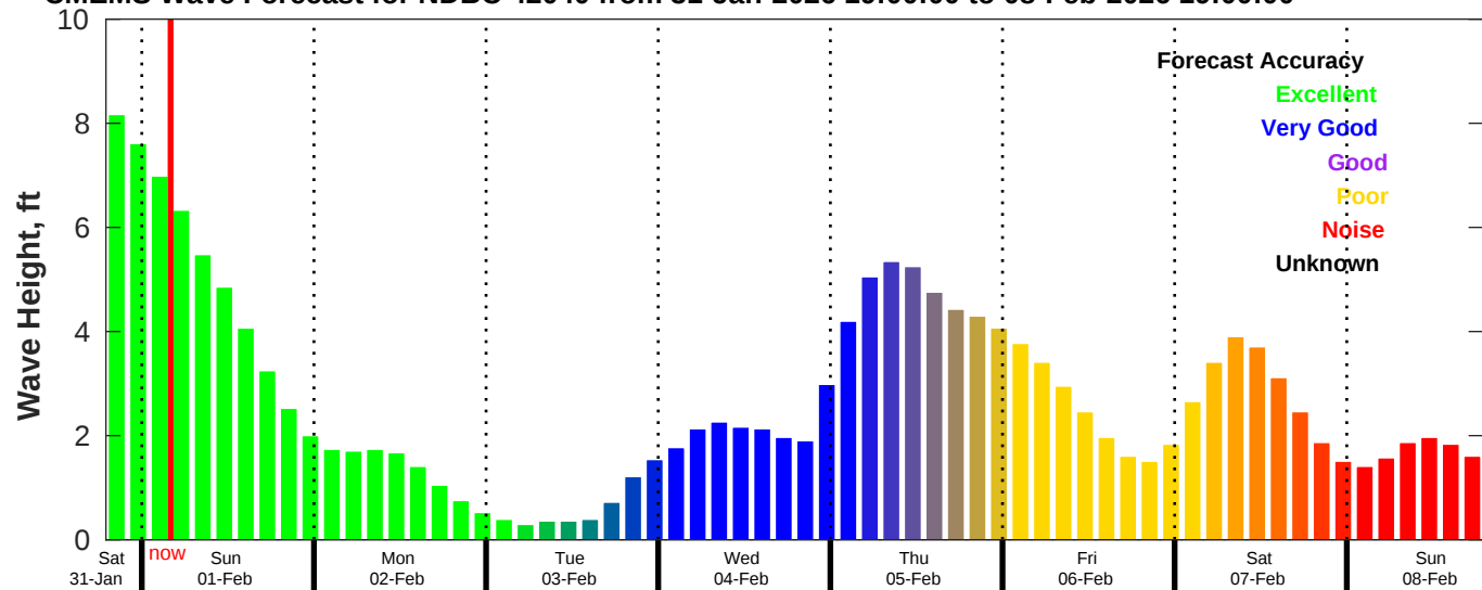
CMEMS Wave Forecast for NDBC 42040 from 31-Jan-2026 19:00:00 to 08-Feb-2026 19:00:00
