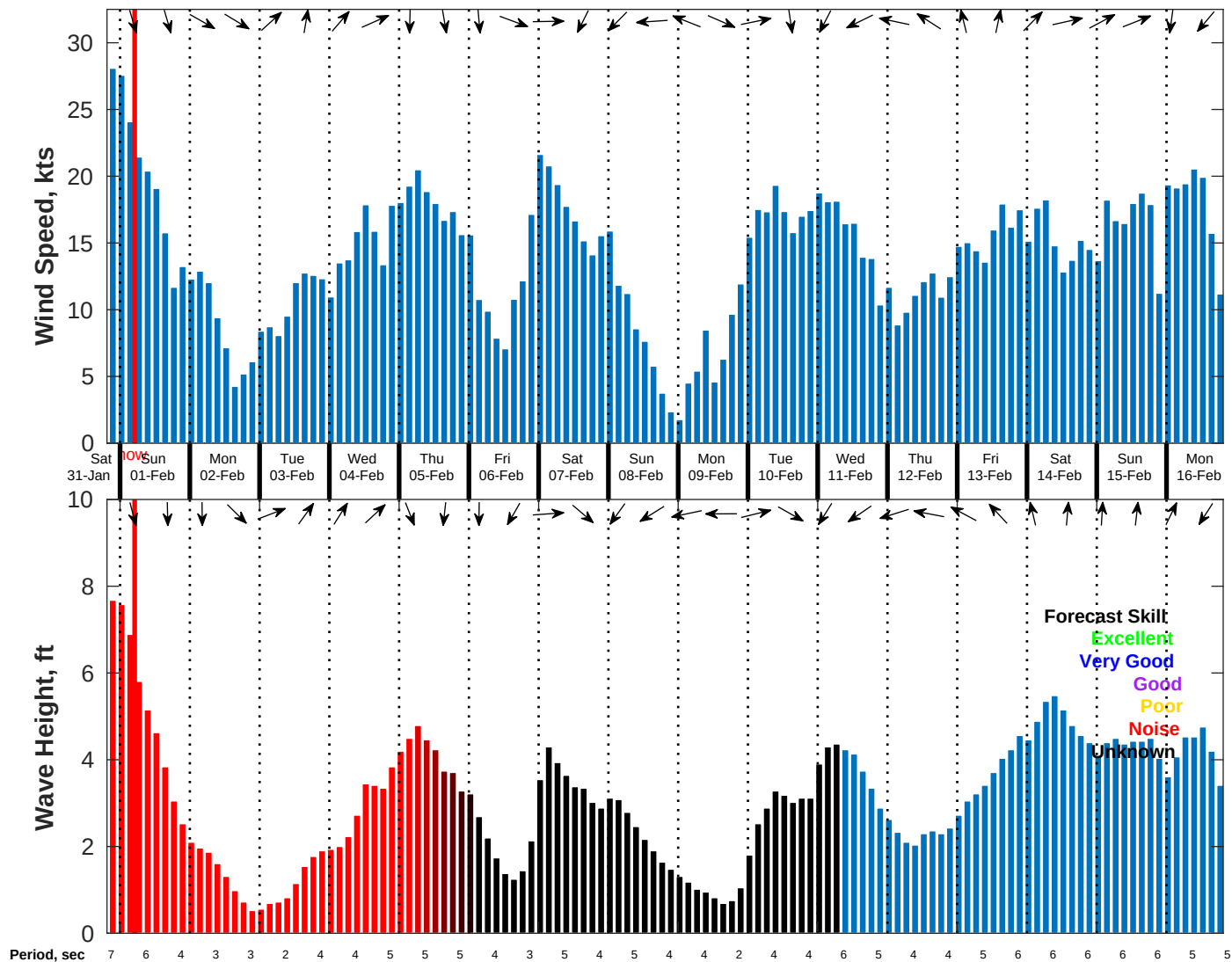
Wind & Wave Forecast for NDBC 42058 from 31-Jan-2026 20:00:00 to 16-Feb-2026 20:00:00
