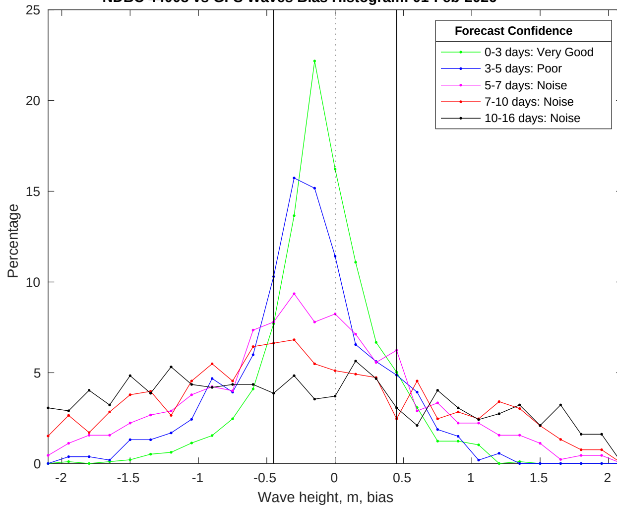
NDBC 44008 vs GFS Waves Bias Histogram: 01-Feb-2026
