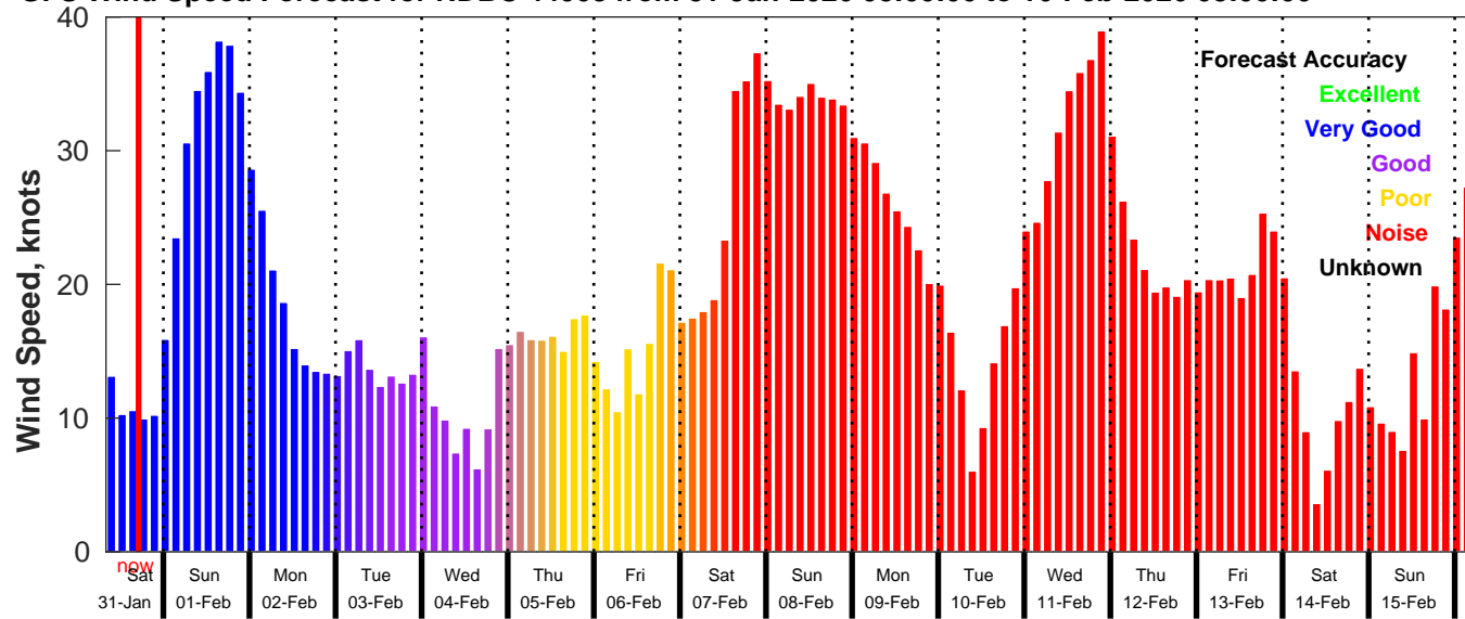
GFS Wind Speed Forecast for NDBC 44008 from 31-Jan-2026 08:00:00 to 16-Feb-2026 08:00:00
