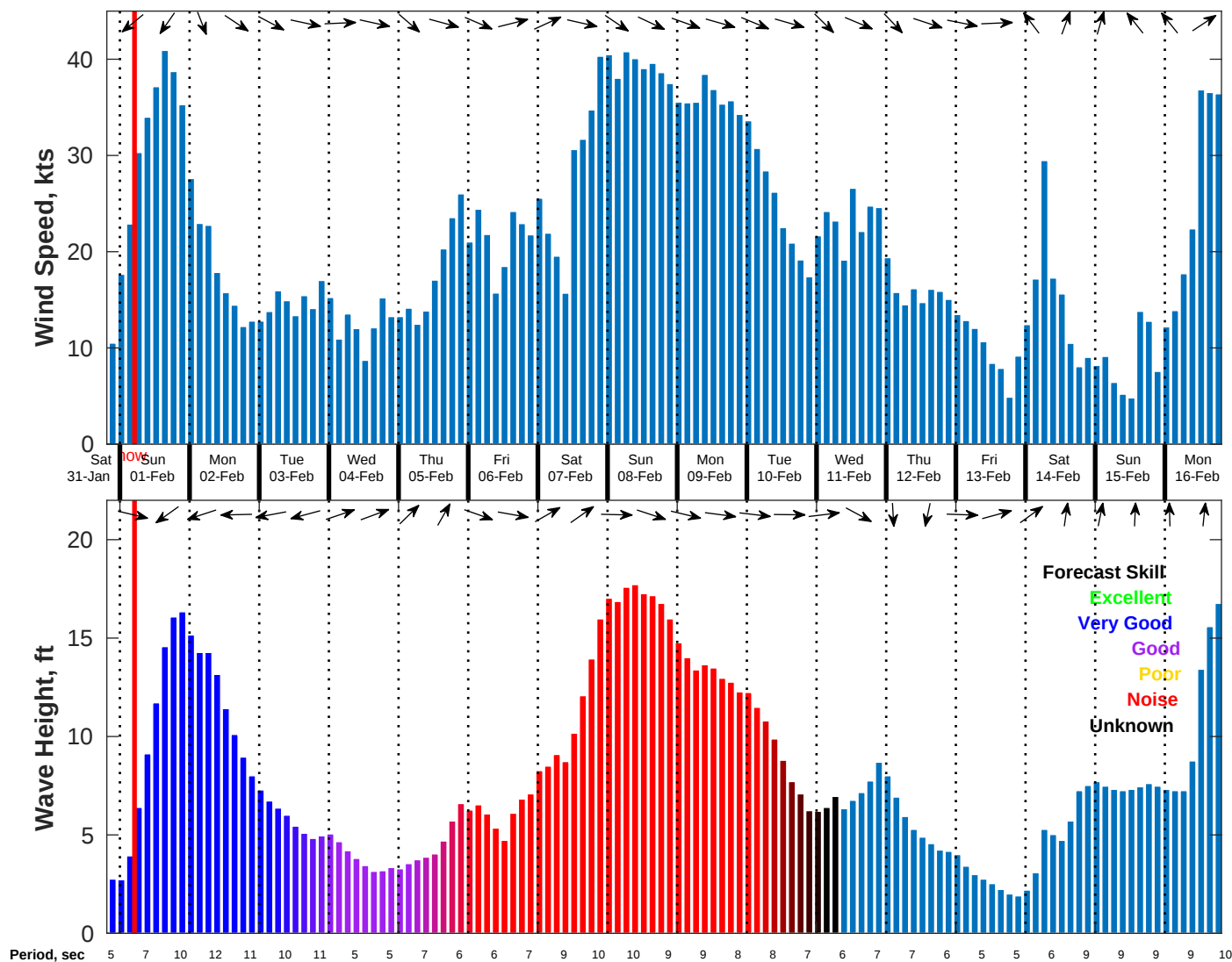
Wind & Wave Forecast for NDBC 44008 from 31-Jan-2026 20:00:00 to 16-Feb-2026 20:00:00
