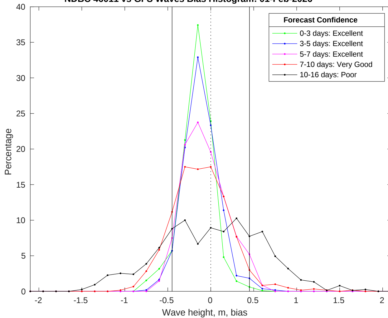
NDBC 46011 vs GFS Waves Bias Histogram: 01-Feb-2026
