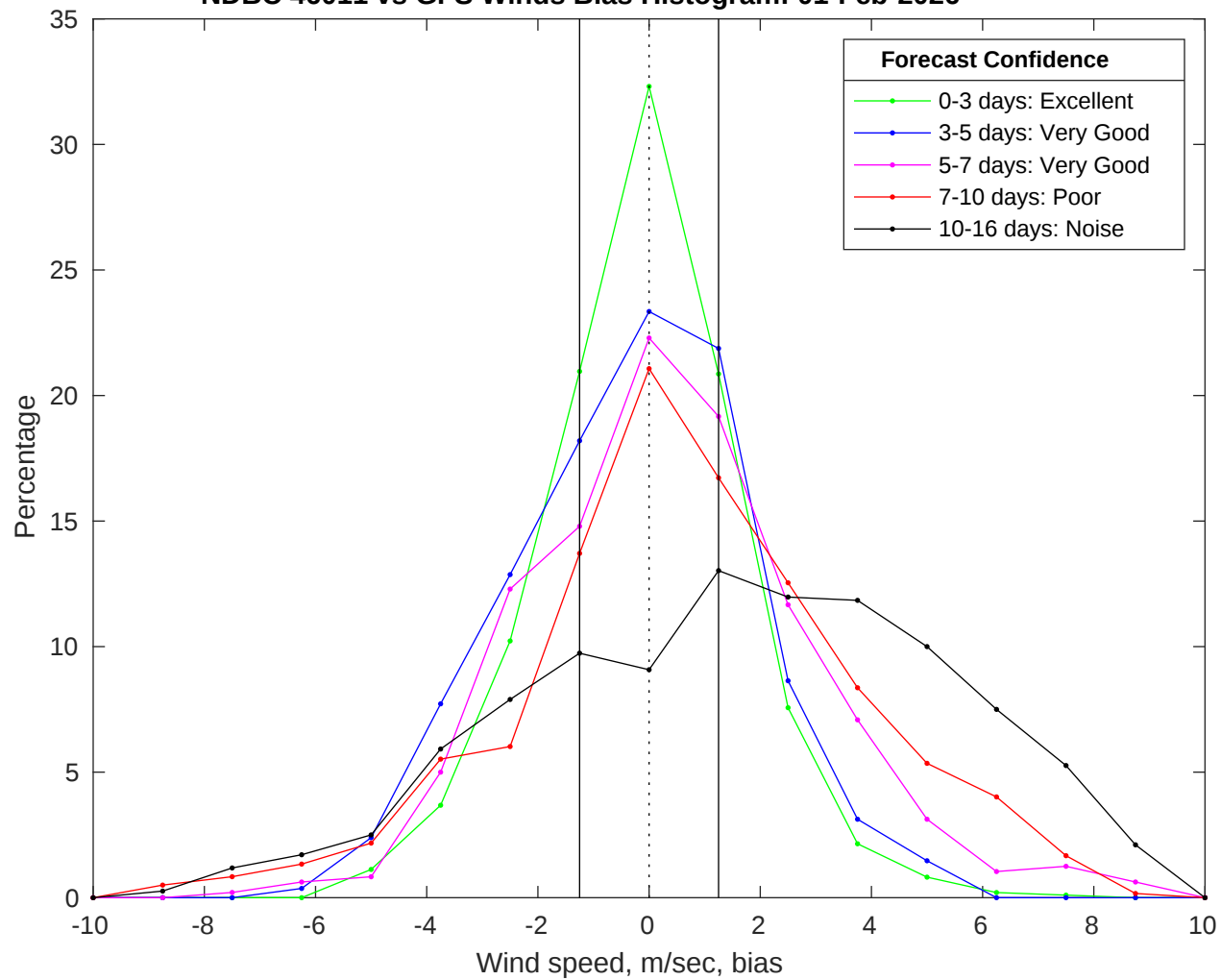
NDBC 46011 vs GFS Winds Bias Histogram: 01-Feb-2026
