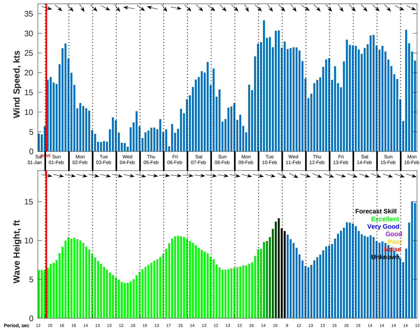
Wind & Wave Forecast for NDBC 46028 from 31-Jan-2026 16:00:00 to 16-Feb-2026 16:00:00
